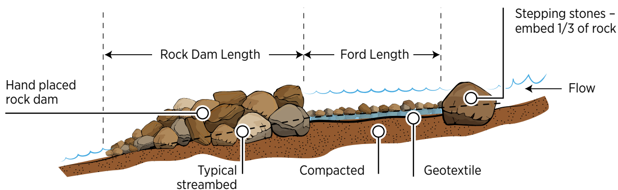
Figure 32: Fords
