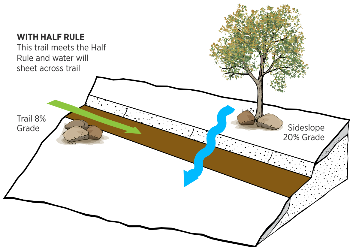
Figure 20: Half rule
