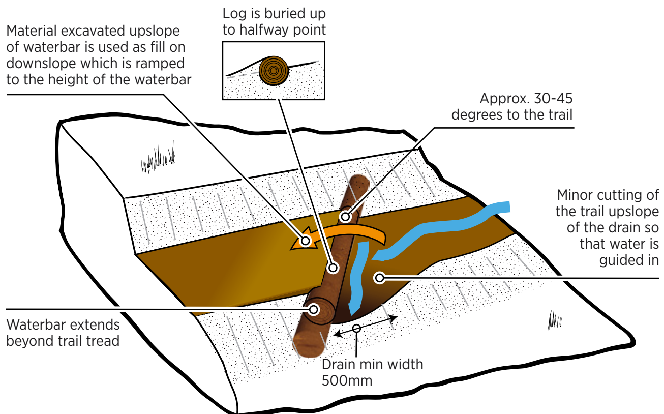
Figure 27: Water bar
