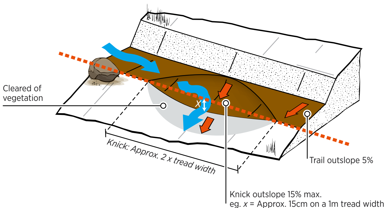
Figure 25: Knicks
