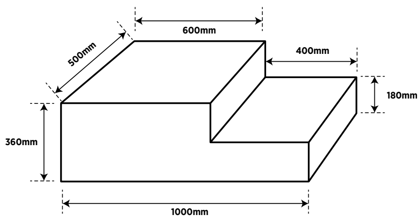
Figure 6: Constructed mounting step
