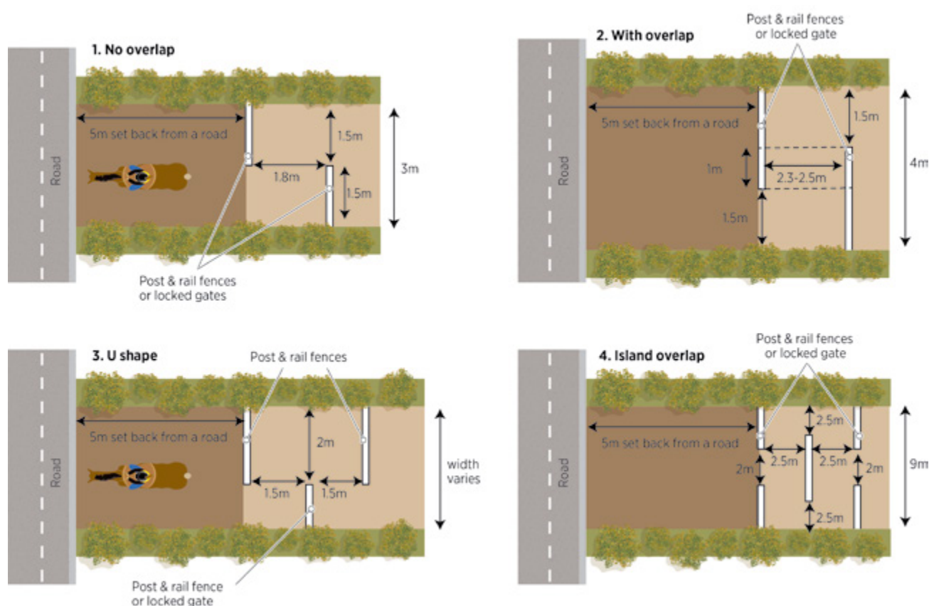
Figure 36: Chicanes
