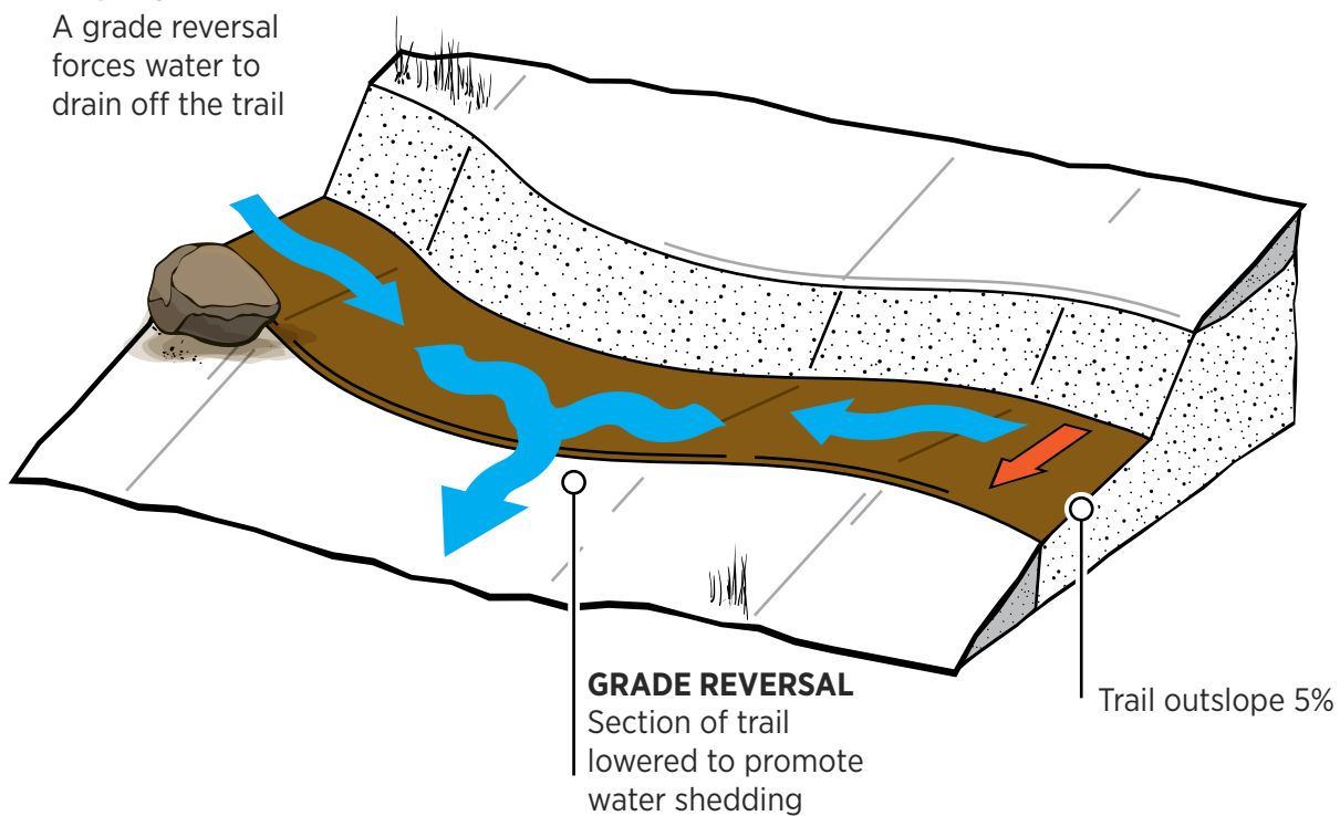
Figure 22: Grade reversal
