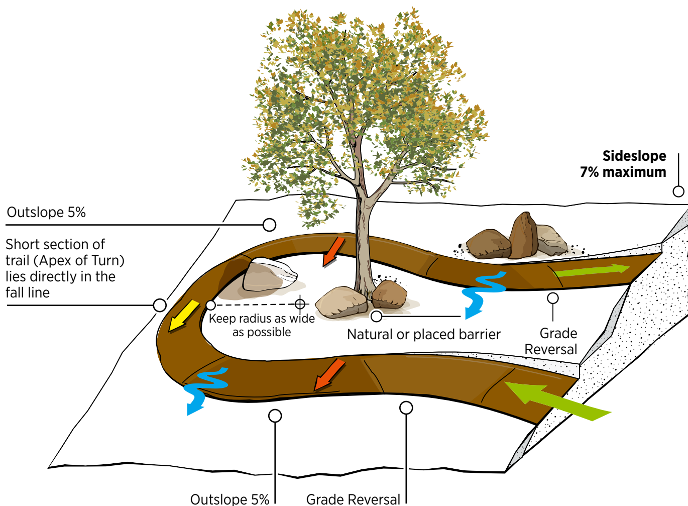
Figure 12: Climbing turn
