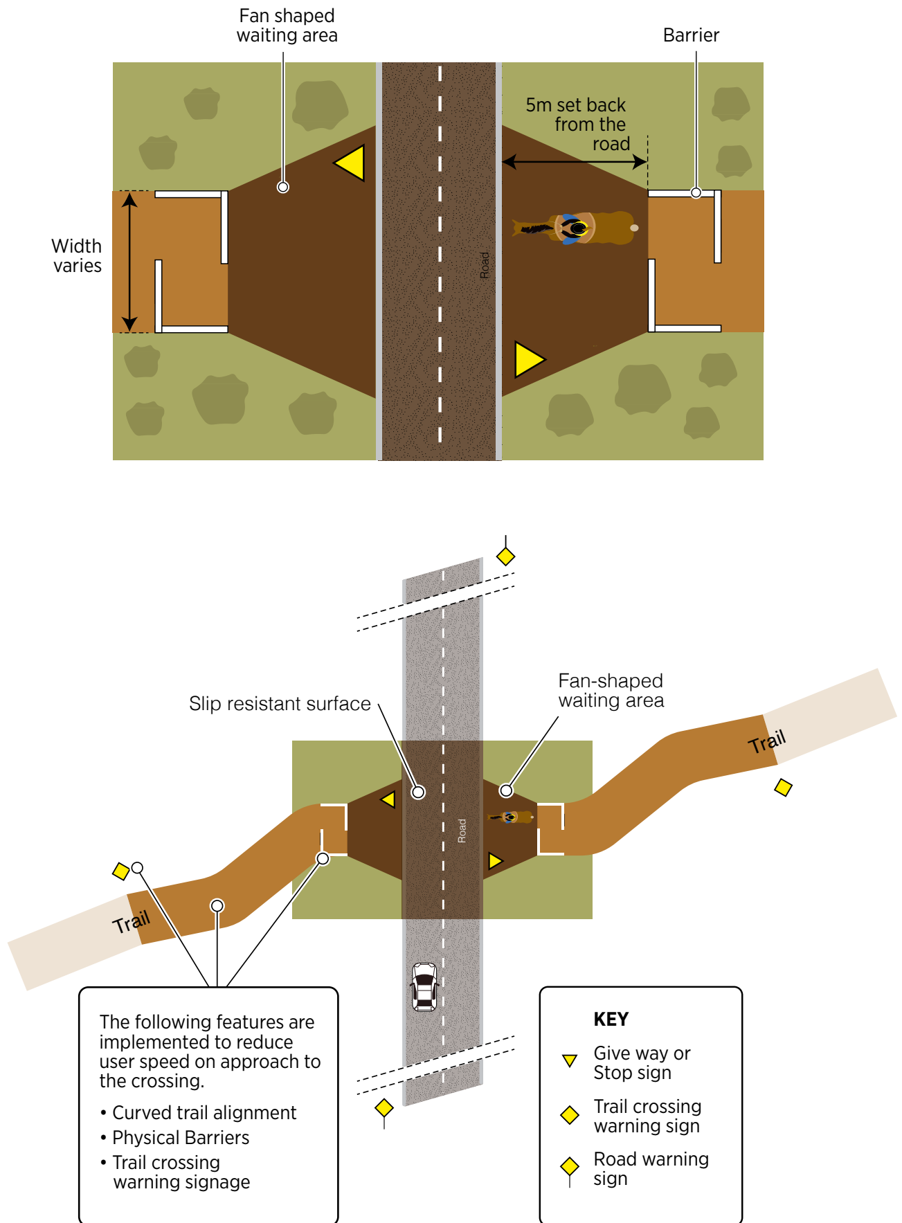
Figure 35: Road crossing sample layout 65
