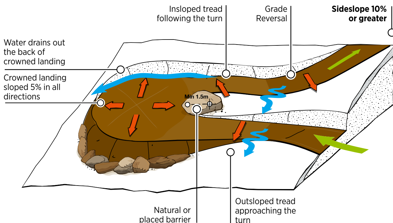
Figure 13: Switchback turn
