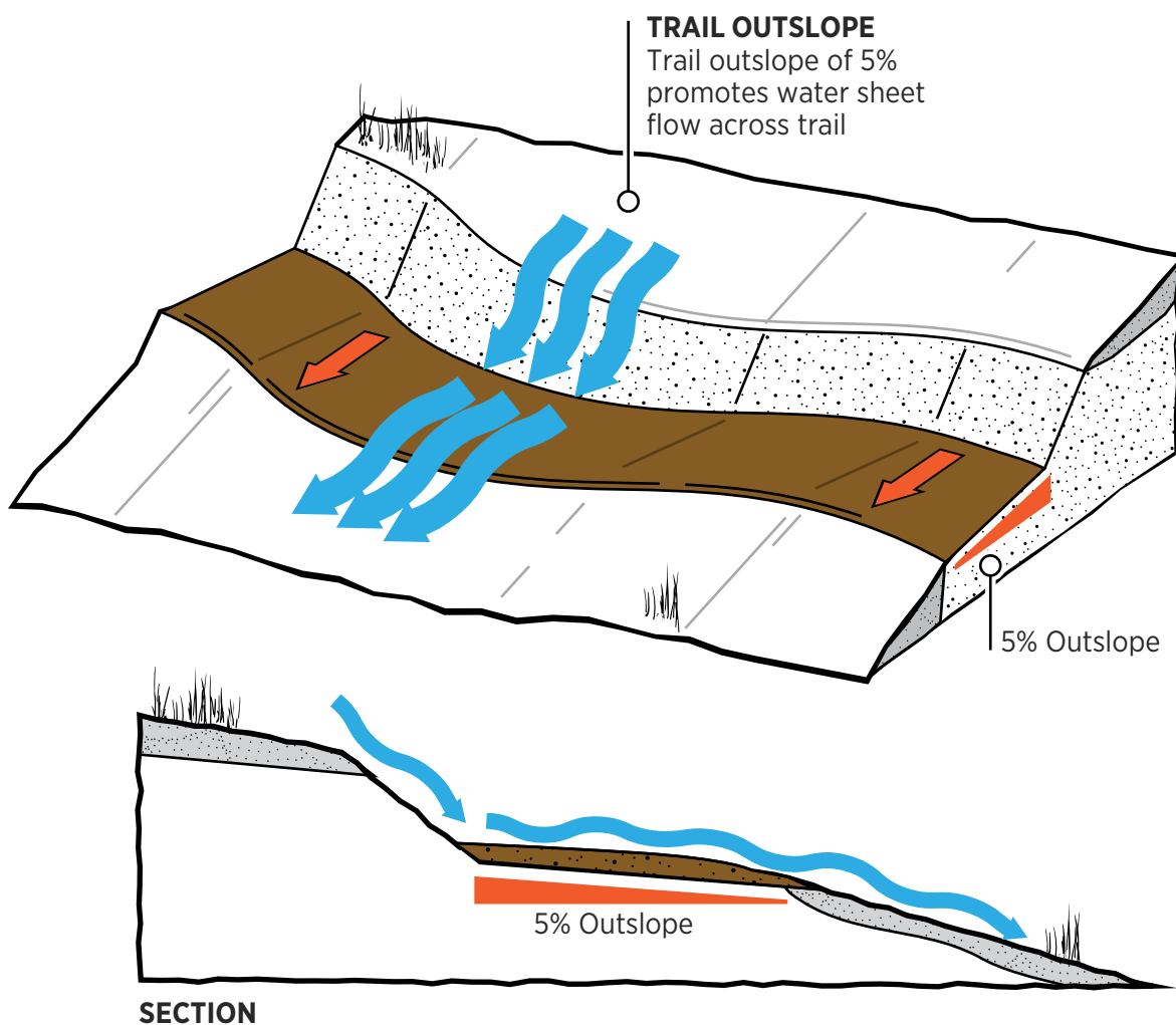
Figure 23: Outslope
