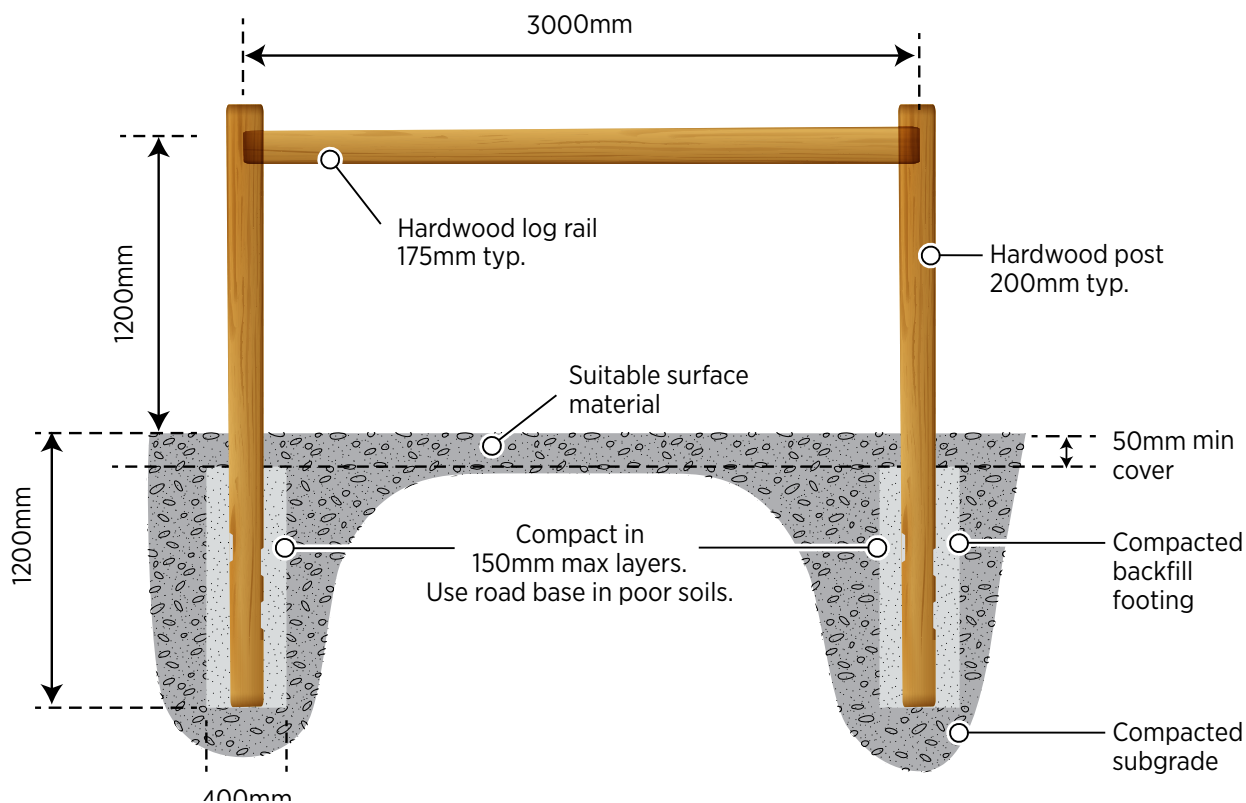
Figure 31: Hitching rails
