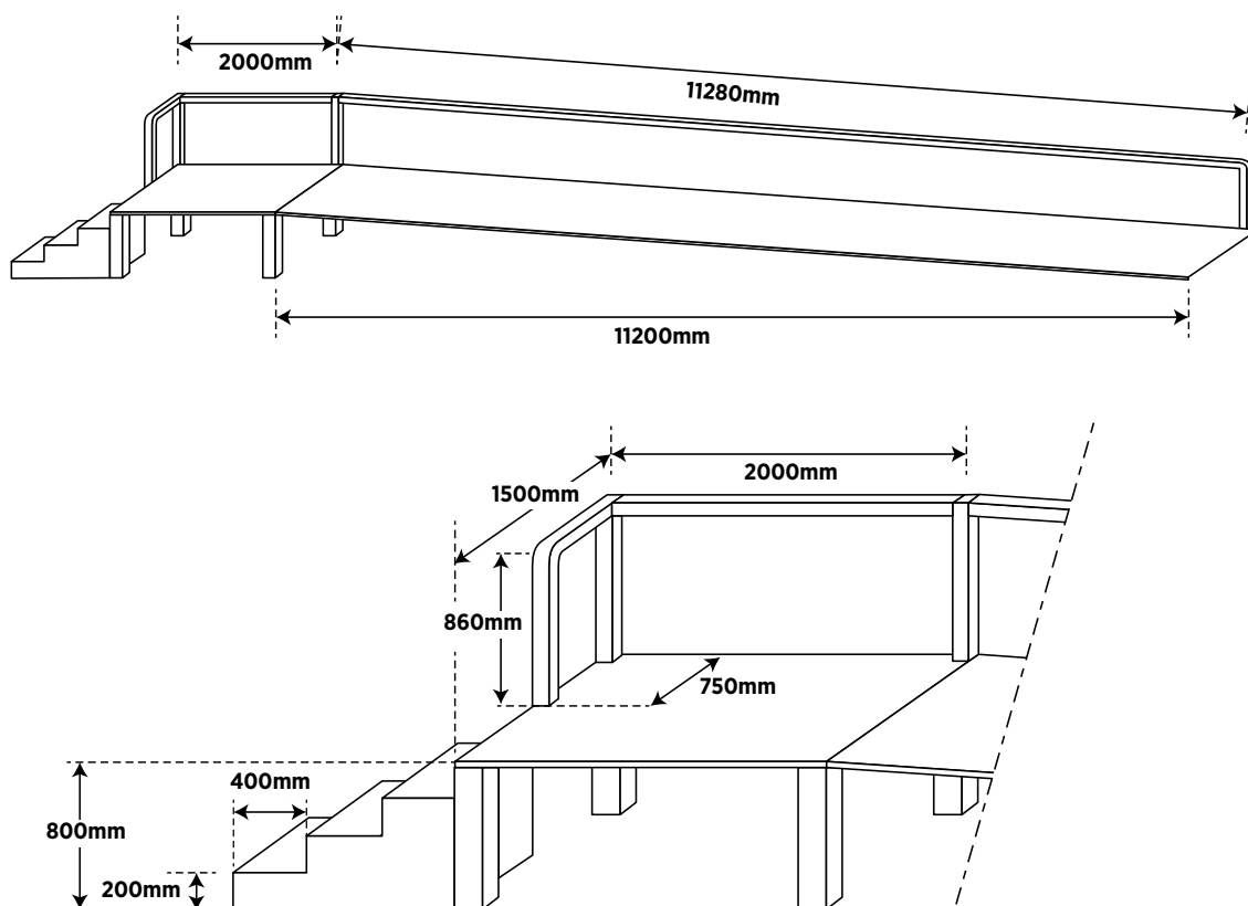
Figure 8: Mounting ramp 29
