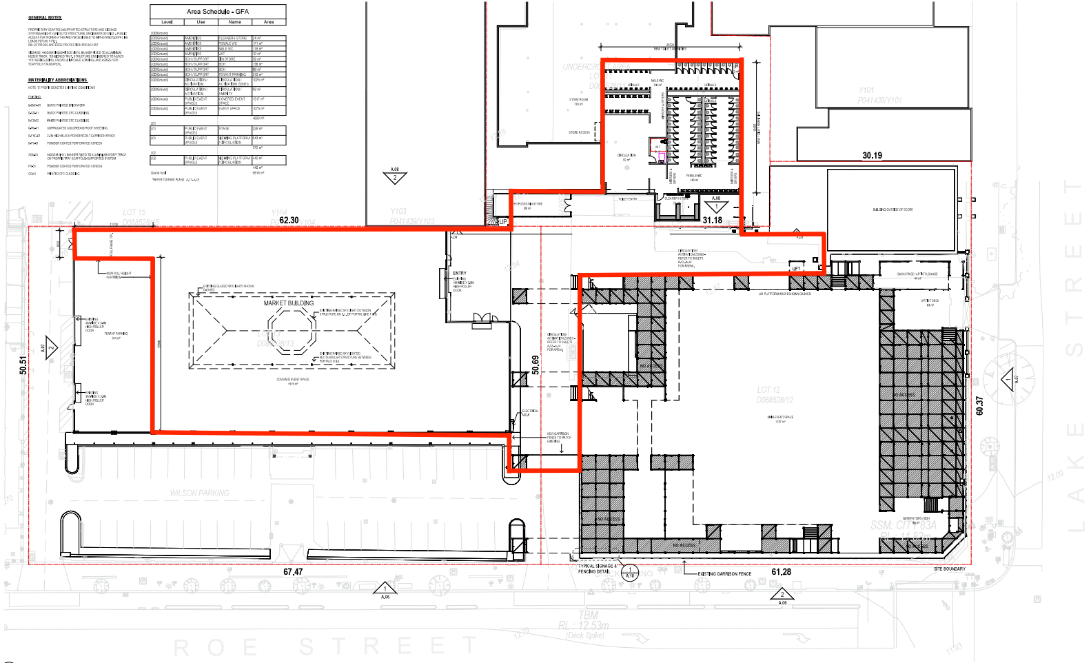
1 PROPOSED PLAN - GROUND
